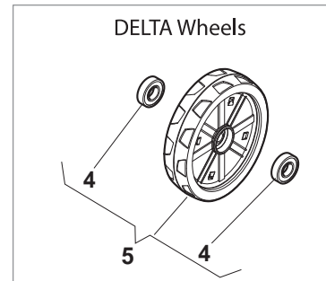
BALL BEARING Version - Ø 200
