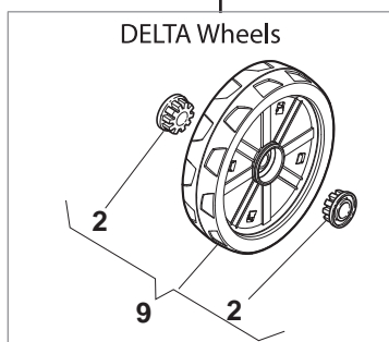
BUSHING Version - Ø 280
