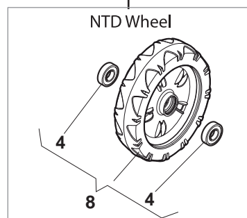
BALL BEARING Version - Ø 280
